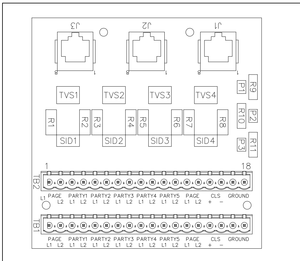
Figure 1. Model 13118-016 TVP Barrier Assembly
